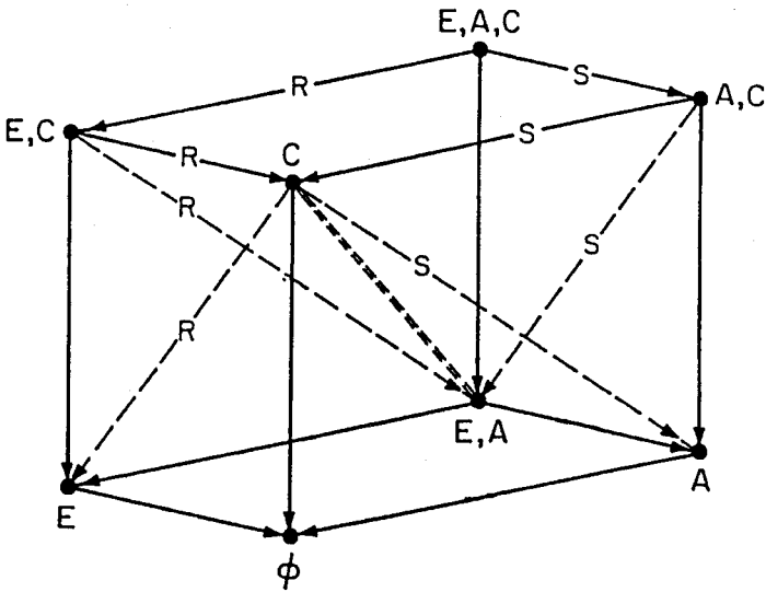
FIG. 3. Summary of results for the \Sigma^\omega case.
