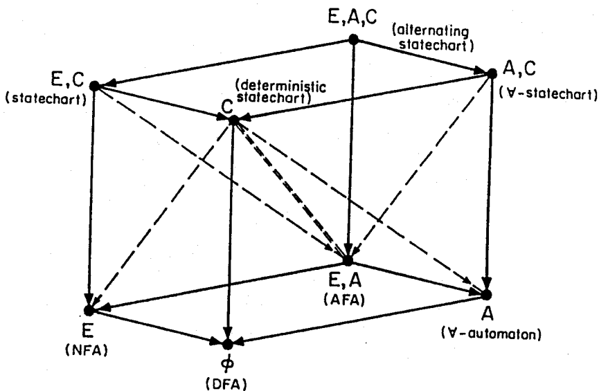
FIG. 2. Summary of results for the \Sigma^* case.
