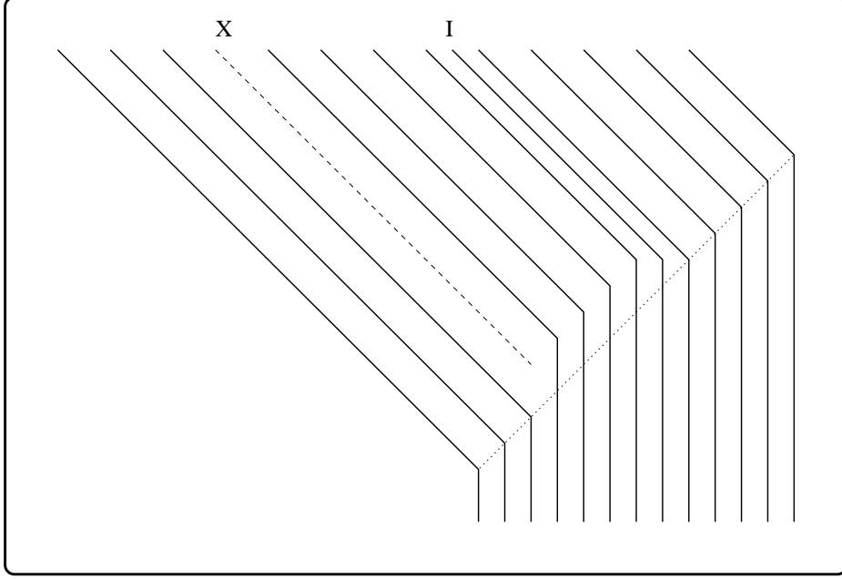
Figure 27: Illustration of (part of) the second third of a block in the \mathcal{D}_2 . An object was omitted from the dashed diagonal segment marked X and inserted in the diagonal segment marked I. The evolution itself is according to the rule. The dotted diagonal indicates the stopping time of moving objects in the corresponding evolution of \mathcal{D}_1 .
