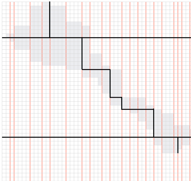
Fig. 3. Decomposition of a partial matrix into staircase matrices (defined by solid thick black lines) and into blocks of consecutive columns with the same defined entries (indicated by thin vertical red lines).
