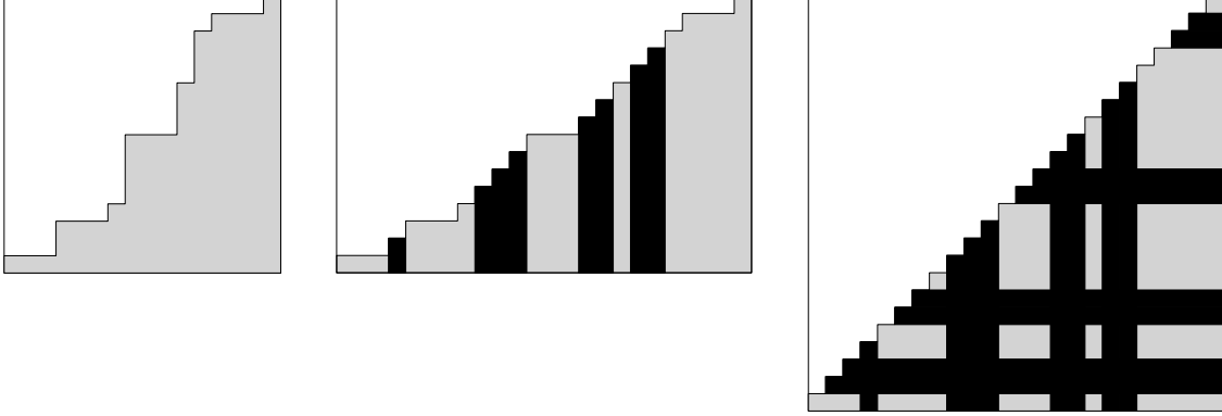
Fig. 2. A staircase matrix M is transformed into a triangular matrix M' in two steps by duplicating columns and rows. Defined entries are gray, undefined white, and duplicated columns/rows black.
