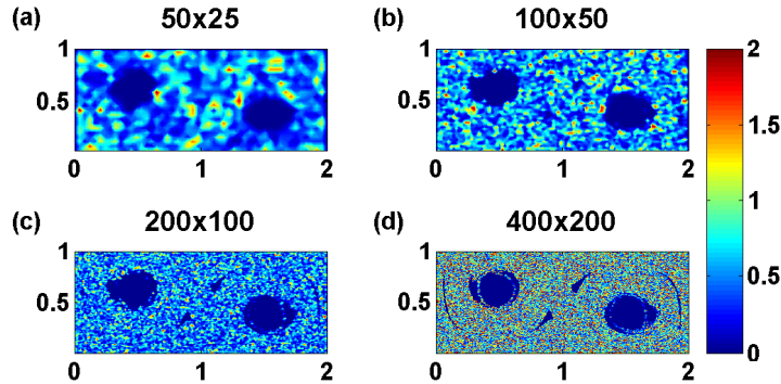
FIG. 7. Dependence on spatial resolution of the Relative Dispersion field. The same 4 resolutions as in Fig. 6 are used to calculate the RD field. The spurious patchiness at the two lowest resolutions (a,b) hides the existence of the small CS structures near x = 1 - these do appear in the lowest resolution of the Max. extent plots Fig. 6a,b. Here A = 0.17, \epsilon = 0.25, \omega = 2\pi/10 .
