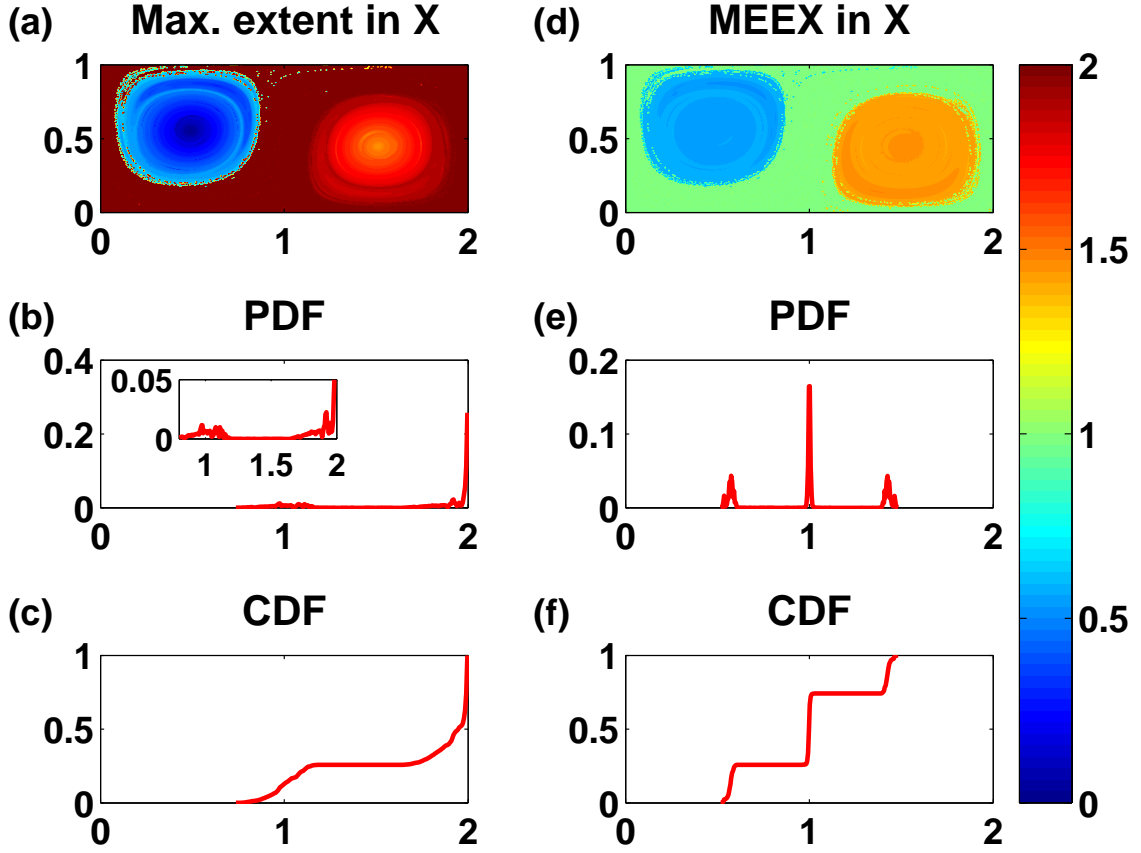
FIG. 3. Oscillatory double gyre - the maximal extent and the extremal mean in x : M_{(1,0)}^+ , M_{(1,0)}^{mean} , their PDF, CDF. In the CDF of M_{(1,0)}^+ , the two gyres appear as two parabolic segments starting near the x values 0.8 and 1.7 whereas the mixing layer appears as a sharp jump at x = 2 , so these three structures are clearly distinguishable in this CDF, whereas in the PDF the high concentration of the distribution function in the mixing layer bin ( x_{max} \lesssim 2 ) makes the contributions to the regular coherent structures hardly detectable (see inset). In the CDF of M_{(1,0)}^{mean} , the two gyres and the mixing layer all appear as sharp jumps, so these three structures are distinguishable, yet their different character is not clearly identifiable. Eq. 10, A = \epsilon = 0.25 , \omega = 2\pi/10 and \tau = 200 .
