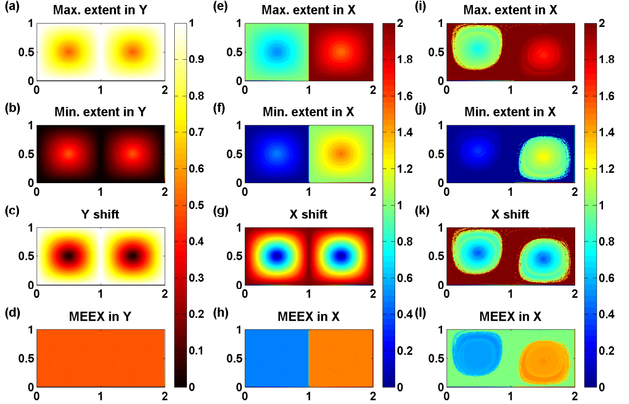
FIG. 2. Two stationary (a-h) and oscillatory (i-l) coherent structures. (a-d) The need to choose resolving direction for obtaining the number of distinct CSs from the corresponding CDFs is demonstrated. The two gyres here have exactly the same extent in the y direction (i.e. identical M_{(0,1)}^{\pm} values) hence the CDF of the M_{(0,1)}^{\pm} does not lead to a distinction between the left and right gyres. (e-h) The need for the maximal/minimal quantifiers is demonstrated - while the maximal/minimal x values ( M_{(1,0)}^{\pm} ) (e,f) distinguish between the right and left gyres, their difference, the maximal shift M_{(1,0)}^{shift} (g), does not. The MEEX in x , M_{(1,0)}^{mean} (h), distinguishes between the gyres yet remains constant throughout the gyre, namely it does not resolve the inner gyre structure. (i-l). The applicability to unsteady flow is demonstrated (Eq. 10 with A = \epsilon = 0.25, \omega = 2\pi/10 and \tau = 200 ). Notice that in both the stationary and oscillatory cases, at the coherent structure centers the fields M_{\mathbf{r}}^{shift}, M_{\mathbf{r}}^+, -M_{\mathbf{r}}^- attain their local minima, whereas M_{\mathbf{r}}^{mean} appears to be approximately constant along each gyre (as a result of the symmetric form of the gyres). In the stationary cases (a,b,e,f) the value of M_{\mathbf{r}}^{\pm} at the center matches the center position whereas in the oscillatory case (i,j) there is a mismatch due to the oscillation: M_{\mathbf{r}}^{\pm} - x_c(t_0; t_0) \cdot \mathbf{r} \neq 0 .
