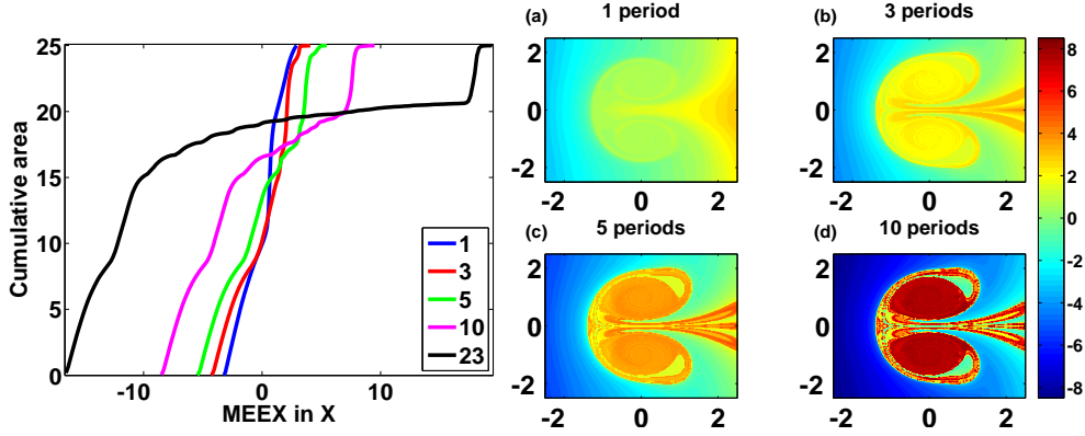
FIG. 8. The MEEEX in X for the OVP open flow at v = 0.25 - dependence on time. The four right panels show the MEEEX in X , M_{(1,0)}^{mean} , at four different extremal windows ( t_1 = 0 , \tau = (1, 3, 5, 10) \cdot 2\pi/\omega ) for the OVP flow (Eq. (11) with \epsilon = 0.2, \omega = 1.45, v = 0.25 ). The left panel shows the CDFs of this flow, multiplied by the area factor of the seeded domain, at the corresponding times - and, the rightmost curve, after 23 periods (see Fig. 9c). The location and size of the vortical core may be identified from the CDFs; The location of the core at different time points corresponds, roughly, to twice (recall that this is the mean of the extrema extents) the x value at which a sharp rise in the CDF occurs (e.g. after 10 periods the vortex is centered near x = 15 ). The area of the fluid carried by the vortices is estimated by the height of this sharp increase in the scaled CDF, namely, the area carried by the vortex after 10 periods is estimated to be \approx 5 . The area of the lobes that are shed from the vortex region correspond to the small wiggles in the CDF. The monotone increase in the CDF up to the lobe shedding regime corresponds to the outer particles that move on average with negative horizontal velocities of approximately -v , with MEEEX value of approximately -v\tau/2 + x_0 + O(1) .
