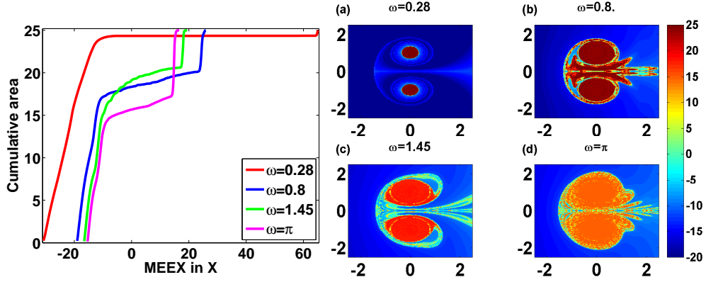
FIG. 9. The CSs dependence on the strain field frequency. On the right panels the MEE in x , M_{(1,0)}^{mean} , is shown for four different frequencies at t_1 = 0, \tau = 100 (about 5, 12, 23 and 50 periods of the corresponding frequencies, notice that in panel (a) the colorbar does not include the extreme, see the CDF for the actual values). The left panel shows the CDF of these fields. The area of the CSs is approximately given by the height of the sharp increased part (i.e. the areas are approximately 7, 5, 5.5, 0.5 for \omega = \pi, 1.45, 0.8, 0.28 respectively). The location is given approximately by double the position of this sharp increase (since we plot the mean and the minimal value here is approximately zero), namely, x_c \approx 30, 35, 50, 135 respectively. The non monotone dependence of the core area on \omega is apparent.
