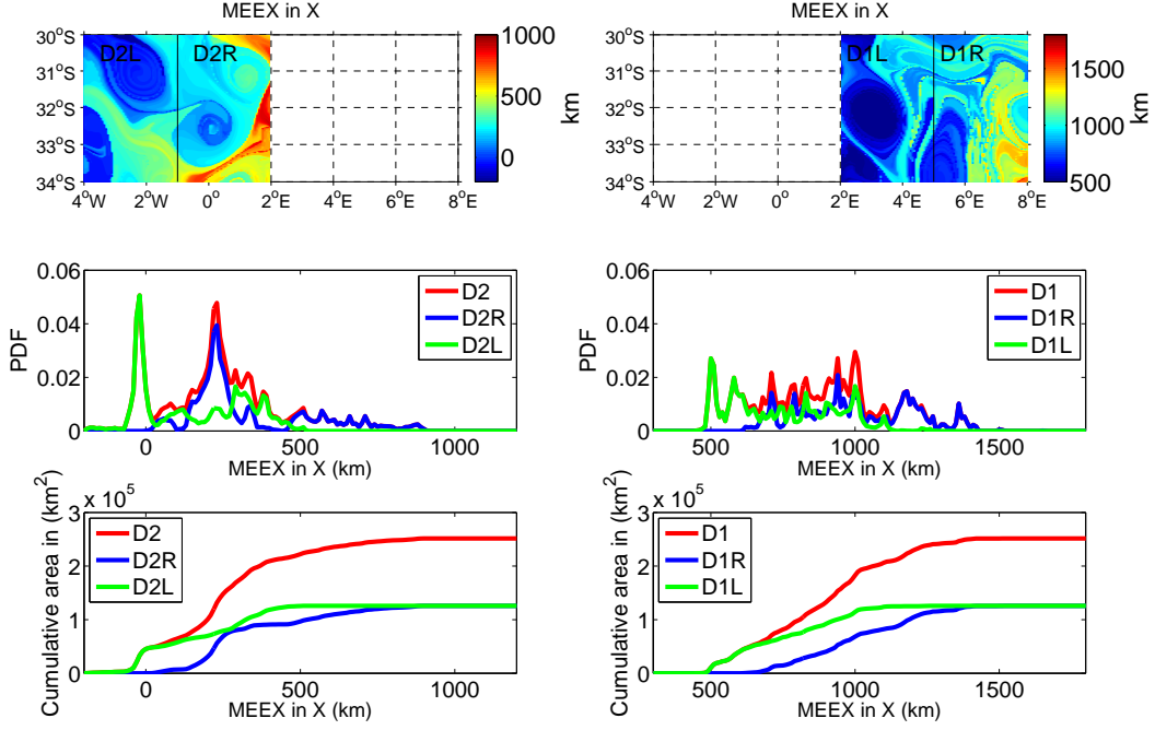
FIG. 16. MEEEX in X for 0-90 days (upper row), PDF (middle row), and CDF (lower row) for different regions and sub-regions of the latitude belt 30^\circ - 34^\circ S . Right column: regions D1 ( 2^\circ E - 8^\circ E , red), and its sub-regions D1L ( 2^\circ E - 5^\circ E , green), and D1R ( 5^\circ E - 8^\circ E , blue). Left column: region D2 ( 4^\circ W - 2^\circ ), red), and its two sub-regions D2L ( 4^\circ W - 1^\circ W , green), and D2R ( 1^\circ W - 2^\circ E , blue). The upper row shows sub-regions of Fig. 14 top-right panel in the regional colorbar.
