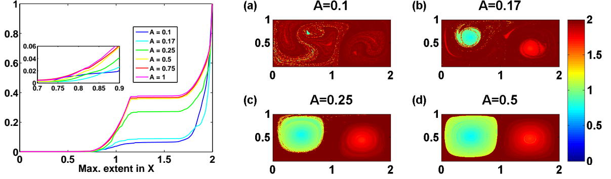
FIG. 4. MET field for the oscillatory double gyre for different base flow intensity A after 20 periods. Right: The maximal extent in x , M_{(1,0)}^+ , is shown for four different base flow strengths. Left: The corresponding CDF for these and additional values of A . The CDF provides succinct presentation of the CSs size and location for the different flows without using any flow visualization analysis. The two gyres and the mixing layer are distinguishable: the left (respectively, right) gyre corresponds to the parabolic increase in the CDF starting near x = 0.75 (respectively, near x = 1.7 ) whereas the mixing layer corresponds to the sharp increase of the CDF near x = 2 . The difference between the location of the gyre center and its maximal value provides information regarding its oscillation magnitude. The accumulated size of the coherent structures is seen to decrease here with decreasing A thus providing estimates for the area of the mixing zone. In all figures \epsilon = 0.25, \omega = 2\pi/10 and t_1 = 0, \tau = 200 .
