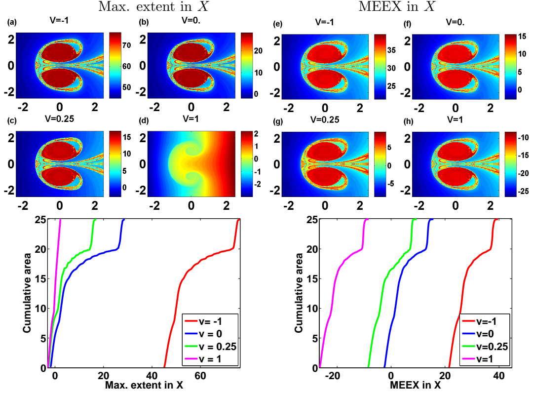
FIG. 12. The MET dependence on translational frame of reference. The OVP flow with the same parameters as in Fig. 8 after 10 periods in four different translational moving frames (Eq. 11 with \epsilon = 0.2, \omega = 1.45 and v = -1, 0., 0.25, 1 at \tau = 10\frac{2\pi}{\omega} ). At v = 0.25 and v = 1 a large portion of i.c. move to the left, the maximal extent for these i.c. is simply their initial horizontal positions, and hence the CDF of the maximal extent does not reflect inherent features of the flow. For v = -1 all i.c. move eventually to the right and the CDF of the max extent field and of the MEEEX, stretched by a factor of two, are identical. Due to this property, we see that the MEEEX CDF has a much weaker dependence on v than the maximal extent CDF.
