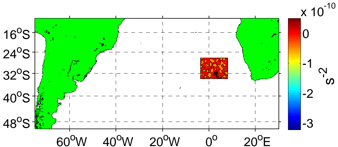
FIG. 13. The South Atlantic region in which particles are seeded on Nov. 24, 2006, is the colored rectangular domain. The colors represent the Okubo-Weiss field (showing some spurious structures 57 ) for Nov. 22, 2006, the closest date to Nov. 24, 2006 for which raw data from the AVISO data set is available.
