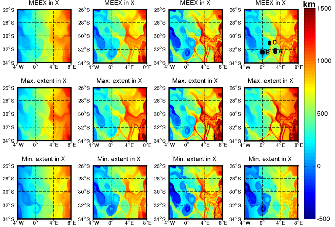
FIG. 14. MEEEX in X (top row), maximal extent in X (middle row) and minimal extent in X (lower row) for a few extremal time windows (columns from left to right): 0-30, 30-60, 60-90, and 0-90 days. The particles were seeded on Nov. 24, 2006. Several separate CSs are identified. The three black dot groups, marked by A-C in the upper-right panel, represent the initial positions of the particle trajectories shown in Fig. 15.
