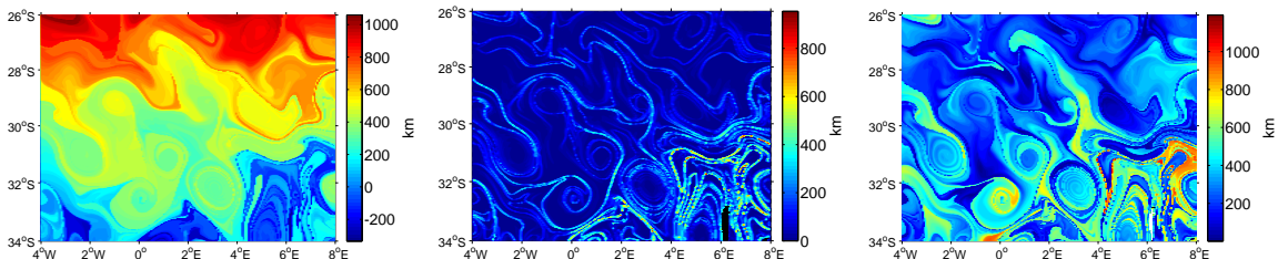
FIG. 18. Additional Lagrangian diagnostics: MEEEX in Y (left), relative dispersion (middle), and absolute dispersion (right) for 0-90 days.
