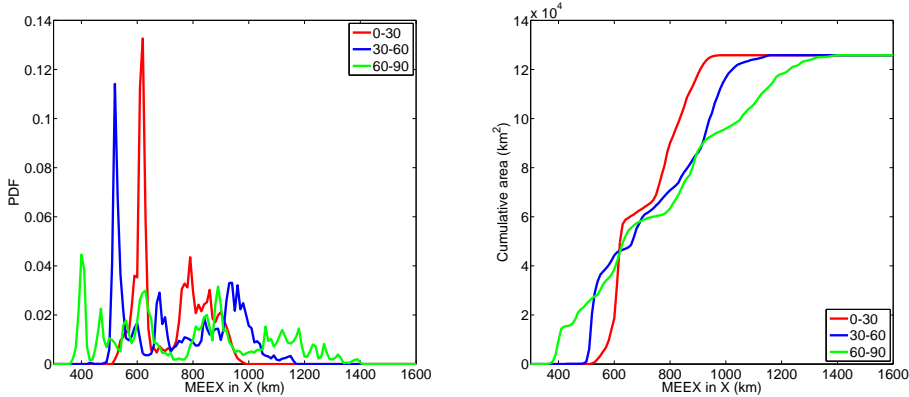
FIG. 17. The PDF and CDF of the MEEEX in longitudinal direction - dependence on time for region D1L. The creation and motion of CS in this region are observed (see text).
