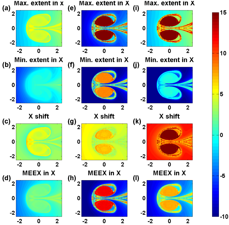
FIG. 11. The four different MET quantifiers for three different extremal windows: (a-d) a 3 periods window starting at t_1 = 0 , (e-h) 3 period window starting at t_1 = 7(2\pi/\omega) , (i-l) 10 period window starting at t_1 = 0 . For t_1 = 0 , (left and right columns) the maximal/minimal extent fields cannot characterize left/right moving trajectories respectively, whereas the MEEEX and shift neutralize this effect. Taking a large t_1 makes the maximal/minimal/mean fields quite similar and resolves this problem (middle column).
