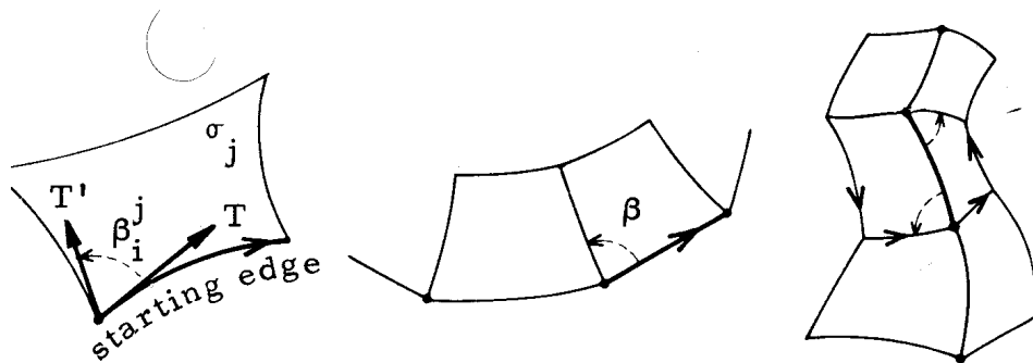
Fig. 8.4 Starting Edges
