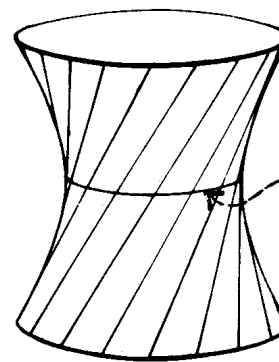
Fig. 2.6 Hyperboloid of Revolution
