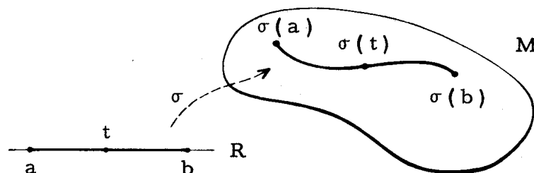
Fig. 1.3 A Curve
