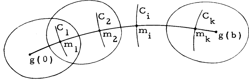
Fig. 10.5 Cross Manifolds
