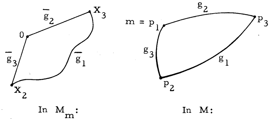
Fig. 10.6 Geodesic Triangle
