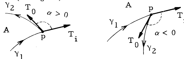
Fig. 8.1 Corner Angles
