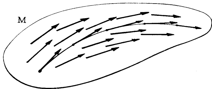
Fig. 1.4 An Integral Curve of a Vector Field
