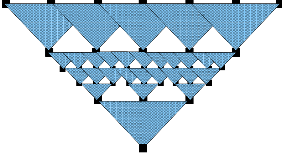
Figure 5: The case of p = 3 (for the proof of Claim 5.3). Smaller triangles replace the three big triangles that would have appeared in the second level. As in Figure 4, only the shaded triangles contain locations that may influence the value of the bottom location.
