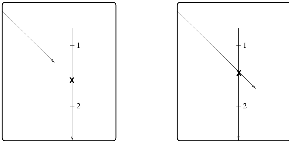
Figure 14: Analysis of Step 3. The left image shows (part of) a diagonal line that stops too early (with respect to its matched vertical line, which starts at either location 1 or location 2), whereas the right image shows a diagonal that stops too late.
