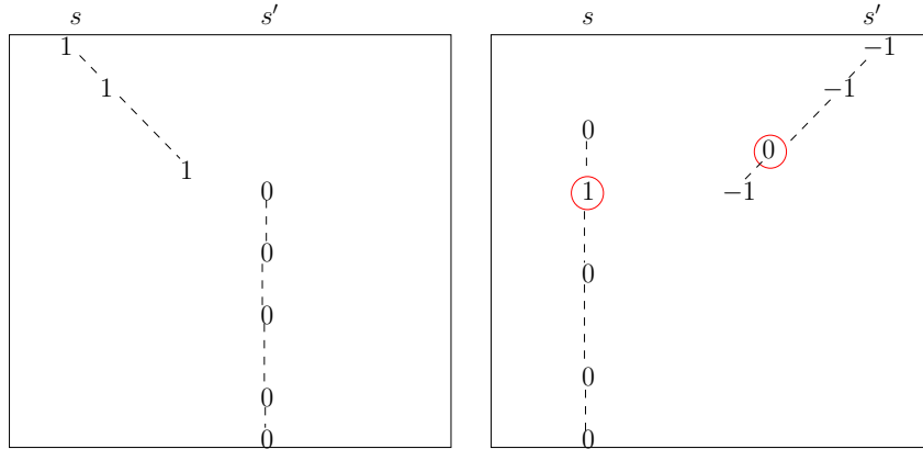
Figure 9: An illustration for Step 2. The left image shows a legal configuration, whereas the right image shows an illegal one. The broken lines indicate the trajectories of the objects, and the violations are circled on the right.
