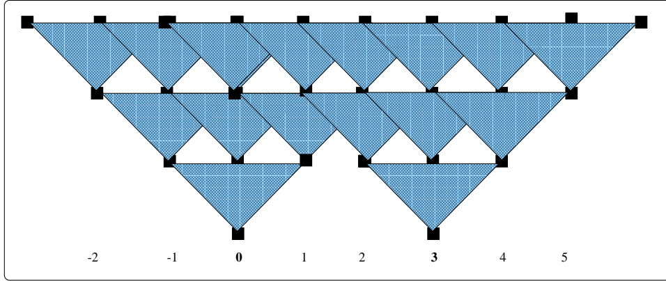
Figure 7: A one-dimensional projection of the case of p = 3 and m = 2 (for the proof of Claim 5.4). The marked positions are scaled by 3^{k-1} . Only the shaded triangles contain locations that may influence the values of the m = 2 bottom locations. The bottom level represents 2^d copies of A_{k-1} , the middle level represents a copy of A_{k-1}^{(6)} , whereas the top level represents a copy of A_{k-1}^{(8)} .
