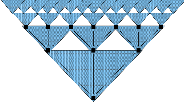
Figure 6: A one-dimensional projection of the case of p = 2 and k' = 3 (for the proof of Claim 5.4). Only the shaded triangles contain locations that may influence the value of the bottom location.
