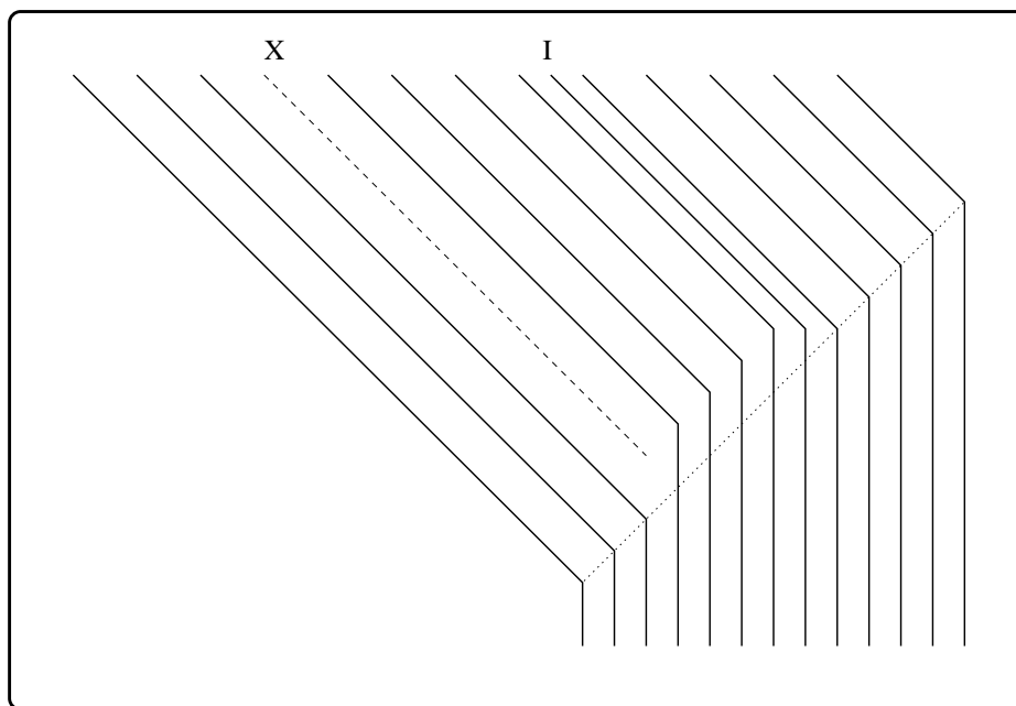
Figure 27: Illustration of (part of) the second third of a block in the second distribution. An object was omitted from the dashed diagonal segment marked X and inserted in the diagonal segment marked I. The evolution itself is according to the rule. The dotted diagonal indicates the stopping time of moving objects in the corresponding evolution of the first distribution.
