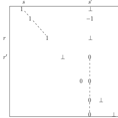
Figure 10: An illustration for the notions of approximate stopping time and approximate time of starting to stand. The object that was in position s at time 0, stopped approximately at time r , and the object who is standing in position s' at time t , started to stand approximately at time r' .
