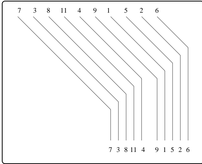
Fig. 26. Illustrating the reliance on the distance measure that counts only changes in the environment function. The objects in the figure start at a (minimal) distance 2 of one another, and (with the exception of lines 4 and 9) they end at distance 1 of one another (leaving no gaps). Note that the gap between lines 4 and 9 cannot be filled without significantly modifying half of the lines in terms of the location function.
