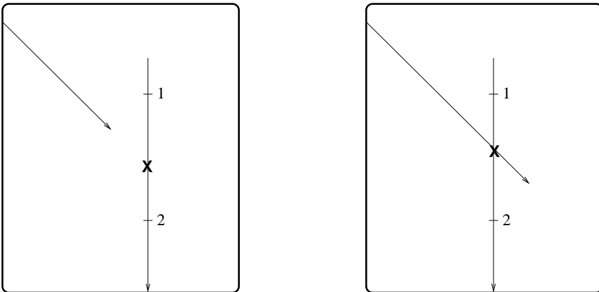
Fig. 14. Analysis of Step 3. The left image shows (part of) a diagonal line that stops too early (with respect to its matched vertical line, which starts at either location 1 or location 2), whereas the right image shows a diagonal that stops too late.
