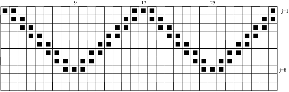
Fig. 1. The saw for k = 16 and n = 32 . (Only 10 time units are shown.)
