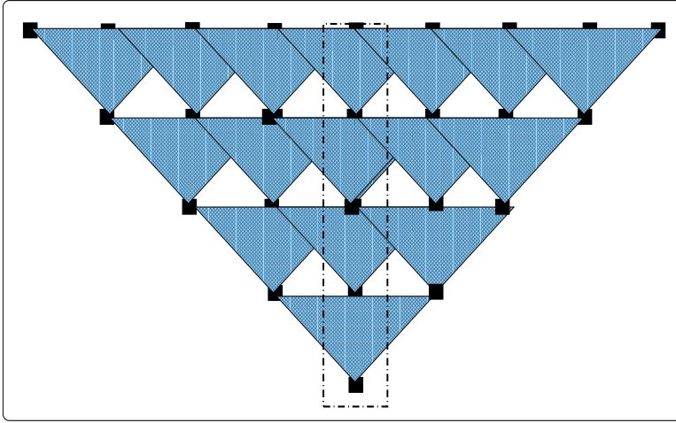
Fig. 8. A one-dimensional projection of the case of t = 4p^\ell (for the analysis of the case of t > n ). Only the shaded triangles (each of height p^\ell ) contain locations that may influence the value of the bottom location. The dashed rectangle marks the boundaries of [t] \times [-(n-1), (n-1)]^d .
