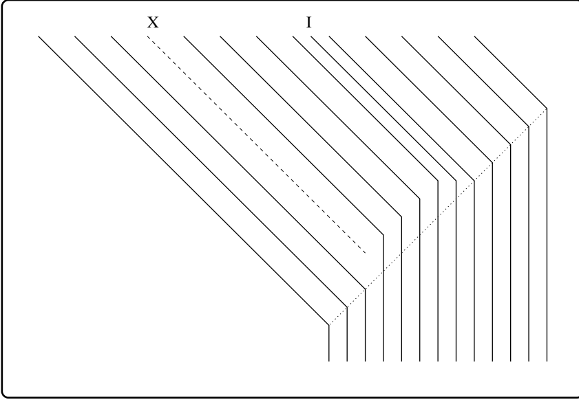
Fig. 27. Illustration of (part of) the second third of a block in the \mathcal{D}_2 . An object was omitted from the dashed diagonal segment marked X and inserted in the diagonal segment marked I. The evolution itself is according to the rule. The dotted diagonal indicates the stopping time of moving objects in the corresponding evolution of \mathcal{D}_1 .
