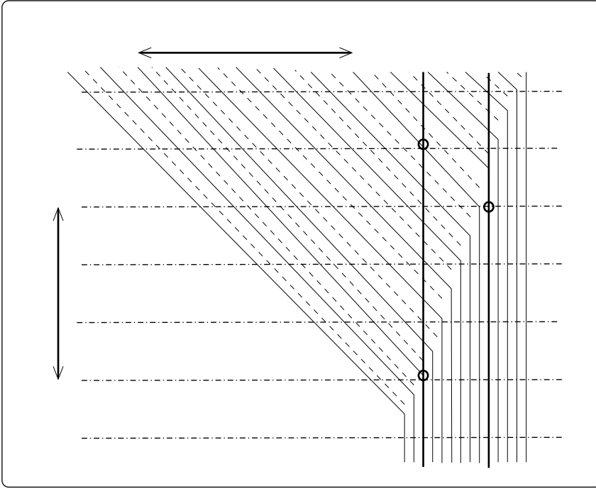
Fig. 25. An illustration for Remark 6.9. The figure shows diagonals that were included in the first set of queries and two vertical lines whose intersections with the horizontal lines were included in the second set of queries. The three small circles indicate intersection points that (together with the first set of queries) provide a proof of illegality of the environment: Too many diagonals (specifically, all diagonals prior to i and subsequent to j ) stop between these two verticals (which can fit only 2/3 of that amount).
