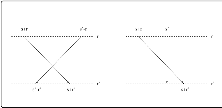
Fig. 11. An illustration for Step 4. The left image shows a crossing of two moving objects, whereas the right image shows an object moving to the right while crossing a standing object (at position s' ).
