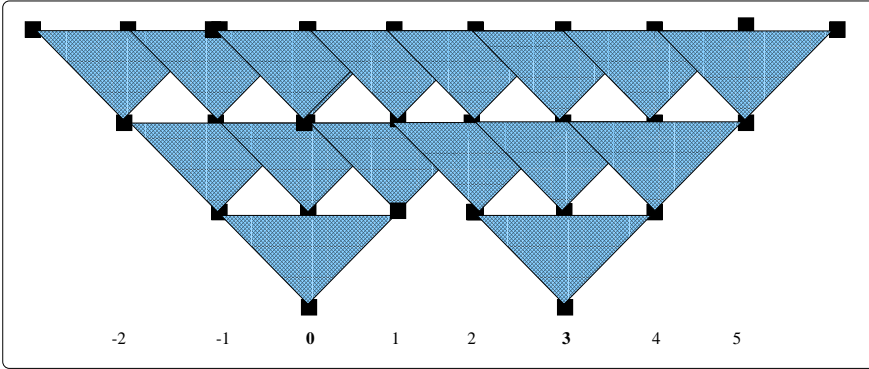
Fig. 7. A one-dimensional projection of the case of p = 3 and m = 2 (for the proof of Claim 5.6). The marked positions are scaled by 3^{k-1} . Only the shaded triangles contain locations that may influence the values of the m = 2 bottom locations. The bottom level represents 2^d copies of A_{k-1} , the middle level represents a copy of A_{k-1}^{(6)} , whereas the top level represents a copy of A_{k-1}^{(8)} .
