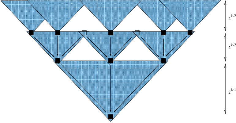
Fig. 4. Demonstrating that A_k < A_{k-1} + 8A_{k-2} (for the proof of Claim 5.2). Only the shaded triangles contain locations that may influence the value of the bottom location.
