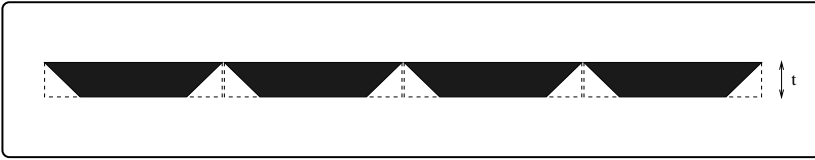
Fig. 21. Tiling a rectangle with trapezoids (for the case of t < \epsilon n/2 ).
