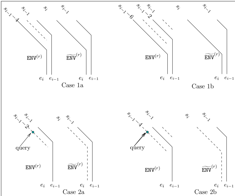
Fig. 23. Detail for the proof of Claim 6.8.4. An illustration for the way the matching is constructed in the illegal region when the queue is empty. As in Figure 22, in the images for \text{ENV}^{(r)} , the dashed lines represent illegal diagonals (in \text{ENV}^{(r)} ), whereas the solid lines represent legal diagonal and vertical segments.
