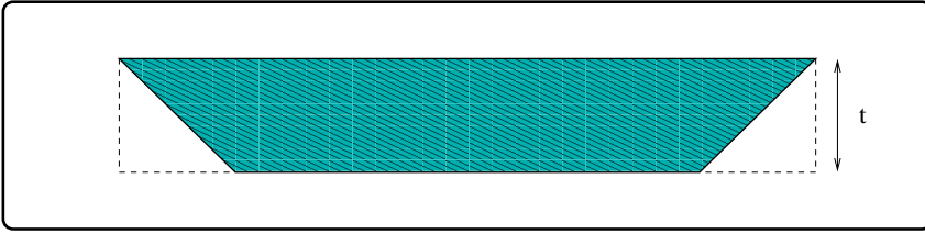
Fig. 20. The trapezoid environments used for the case of t < \epsilon n/2 .
