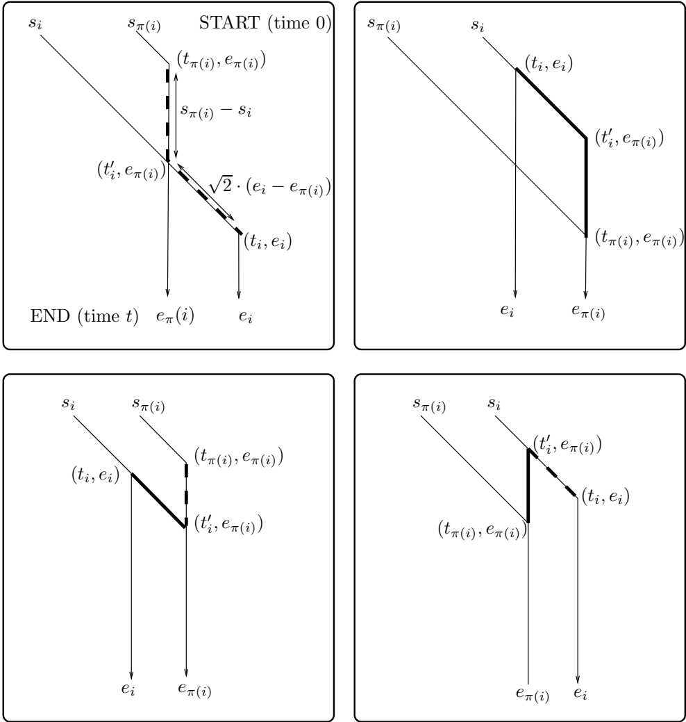
Fig. 16. An illustrations for the charging rule in the analysis of Step 4. The omitted segments are shown in dashes and the added segments are shown bold. In all cases line i is charged for either the omission or the addition of the diagonal segment whose endpoints are (t_i, e_i) and (t'_i, e_{\pi(i)}) and for either the omission or the addition of the vertical segment whose endpoints are (t'_i, e_{\pi(i)}) and (t_{\pi(i)}, e_{\pi(i)}) . The four cases correspond to the four possibilities with respect to the relation between s_i and s_{\pi(i)} and between e_i and e_{\pi(i)} . The lengths of the segments appear in the top left illustration.
