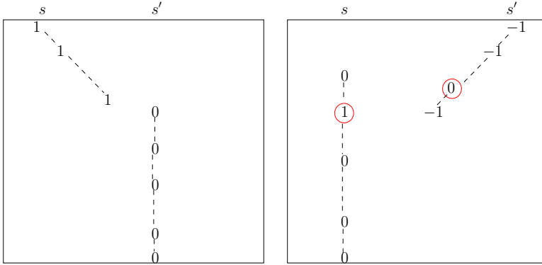
Fig. 9. An illustration for Step 2. The left image shows a legal configuration, whereas the right image shows an illegal one. The broken lines indicate the trajectories of the objects, and the violations are circled on the right.
