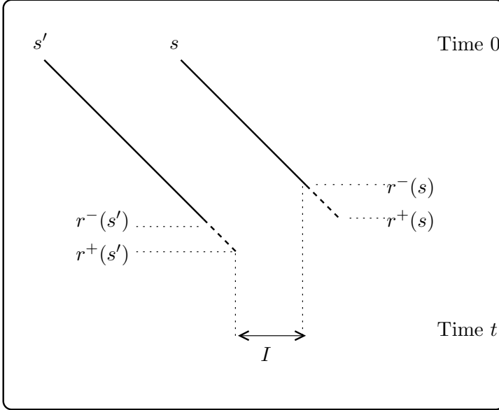
Fig. 13. An illustration for the check performed in Step 5. The solid segments indicate that the object is moving, and the dashed segments indicate that the object is either moving or already stopped. The interval I must fully consist of standing objects at time t .
