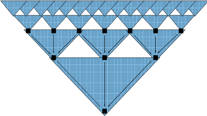
Fig. 6. A one-dimensional projection of the case of p = 2 and k' = 3 (for the proof of Claim 5.6). Only the shaded triangles contain locations that may influence the value of the bottom location.
