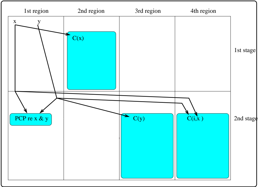
Fig. 3. The evolution of the environment used in the proof of Theorem 4.1, where C denotes the commitment/encoding and i = F(y) . The rounded rectangles represent areas that display values, and the areas outside them (with the exception of areas at the vicinity of arrows) are inactive.
