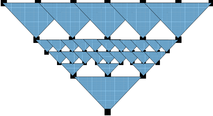
Fig. 5. The case of p=3 (for the proof of Claim 5.4). Smaller triangles replace the three big triangles that would have appeared in the second level. As in Figure 4, only the shaded triangles contain locations that may influence the value of the bottom location.
