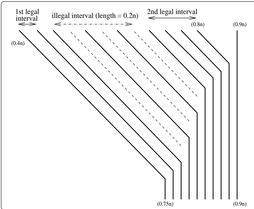
Fig. 22. A generic environment in the family used in the proof of Theorem 6.8. The three dashed lines are illegal (since they have no vertical continuation at the point that they stop). Only a portion of the environment is shown, say [0, 0.4n] \times [0.4n, 0.9n] .
