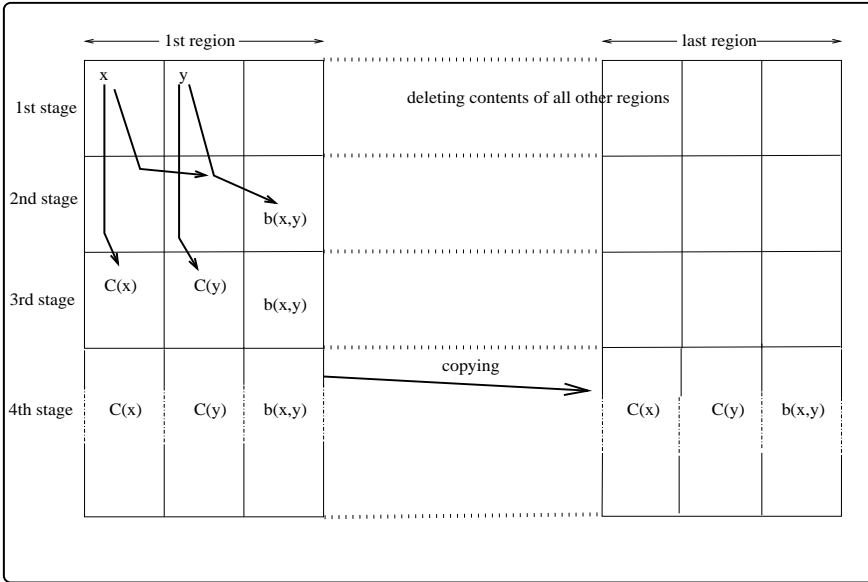
Fig. 2. The evolution of the environment used in the proof of Theorem 3.5. Only the first and last regions are shown; the other regions are identical to the last region.
