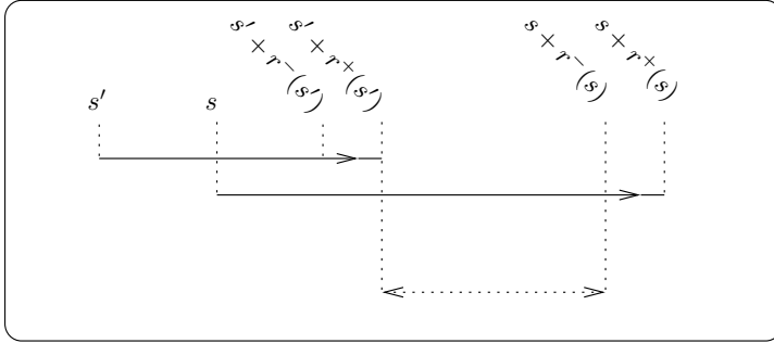
Fig. 17. The intervals considered in Assumption 3. The two arrows depict the actual movement of two objects, starting at locations s' < s . The actual stopping times are within the intervals (s' + r^-(s'), s' + r^+(s')) and (s + r^-(s), s + r^+(s)) , respectively. The interval [s' + r^+(s'), s + r^-(s) + 1] is depicted by a dotted double-arrow.
