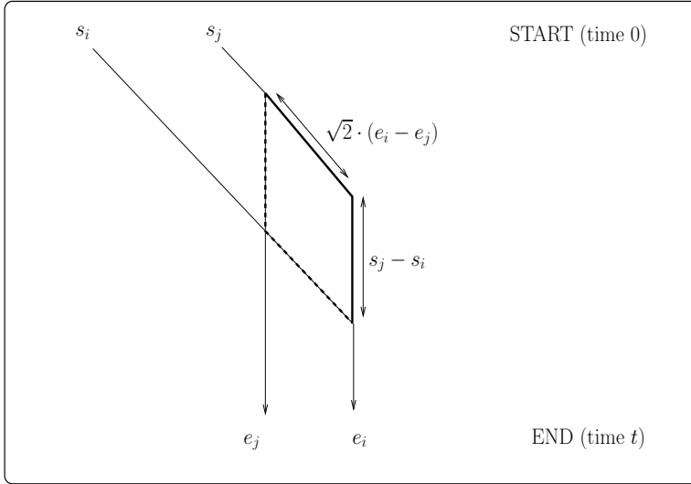
Fig. 15. Eliminating a crossing between lines i and j in the analysis of Step 4 for the case that \pi(i) = j and \pi(j) = i . The segments that are omitted are shown in dashes, and the segments that are added are shown in bold.
