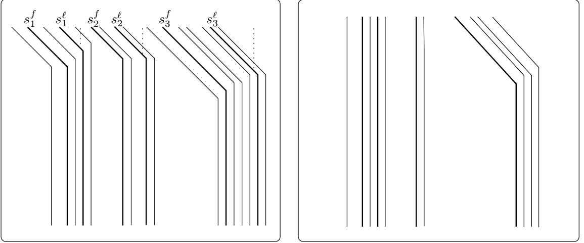
Fig. 18. An illustration for modifications performed in Stage I of the analysis of Step 5. The left image shows (part of) the environment \text{ENV}^I before lines are removed or “straightened”, whereas the right image shows the environment after these changes. The illustration shows three connected components C_j , where C_1 and C_2 are short, while C_3 is long. The notation s_j^f stands for s_{\min}(C_j) , and s_j^l stands for s_{\max}(C_j) . Lines starting at the corresponding six positions are bold. The dotted lines indicate the positions s_j^l + r^-(s_j^l) + 1 . Since C_1 and C_2 are both short, no lines are removed “between” them, while since C_3 is long all lines “between” C_2 and C_3 are removed, as well as the lines “at the end” of C_3 . Finally, all (remaining) lines in the short buckets C_1 and C_2 are turned into vertical lines.
