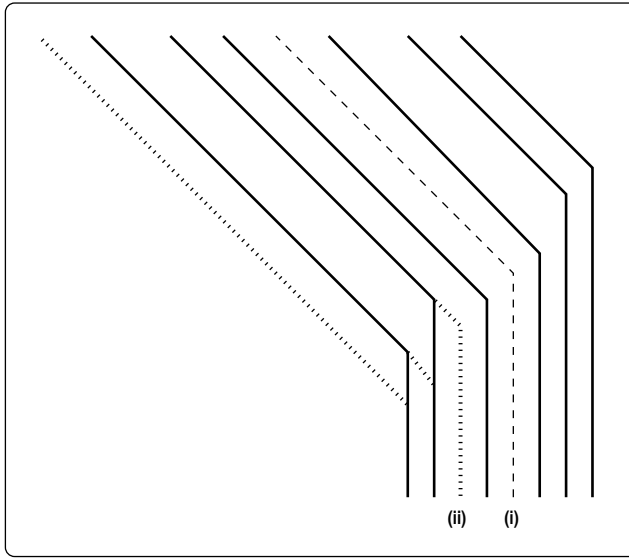
Fig. 19. Filling up the vertical gaps in the analysis of Step 5. The original lines are shown in solid, the dashed line at location (i) is inserted without conflicts, whereas the dotted lines show an insertion at location (ii) and its propagated corrections.
