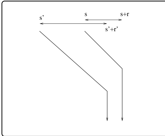
Fig. 12. An illustration for Step 5. The first object moves from position s to position s+r , where it stops, whereas the second objects moves from s' < s to s'+r' \in [s, s+r] . In this case, the interval [s'+r', s+r] must be filled with stopping objects (at time t ).
