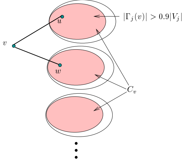
Figure 4: An Illustration for the proof of Claim 4.3.2, Case 2.1.
