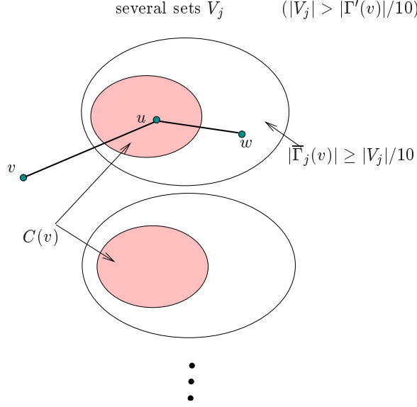
Figure 7: An Illustration for the 2nd subcase of Case 2.2 in the proof of Claim 4.4.2.
