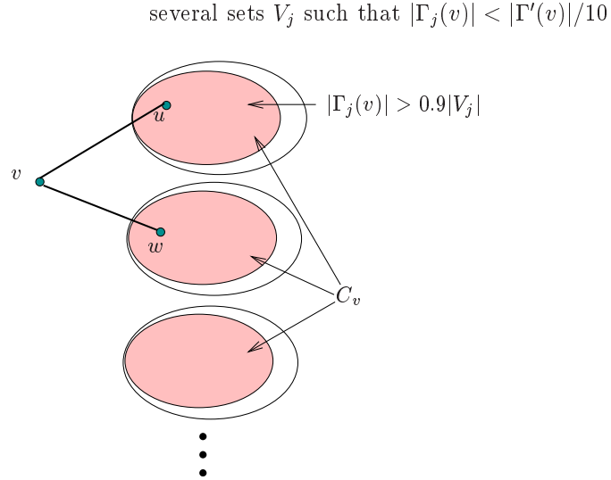
Figure 6: An Illustration for Case 2.1 in the proof of Claim 4.4.2.
