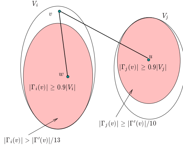
Figure 5: An Illustration for the 1st subcase of Case 1.2 in the proof of Claim 4.4.2.
