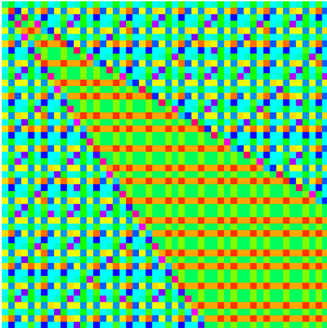
Fig. 8. Upper-left corner of \psi^\omega(a) where the 26 symbols have been replaced with different colors. (Colors are only available on the Web version of this article.)
