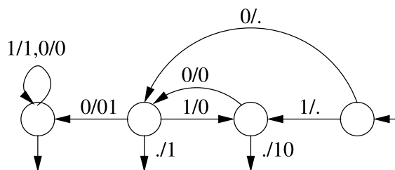
Fig. 6. The successor function for the Fibonacci system.
