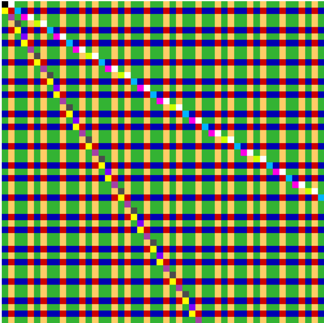
Fig. 7. Upper-left corner of \varphi^\omega(a) where the 13 symbols have been replaced with different colors. (Colors are only available on the Web version of this article.)
