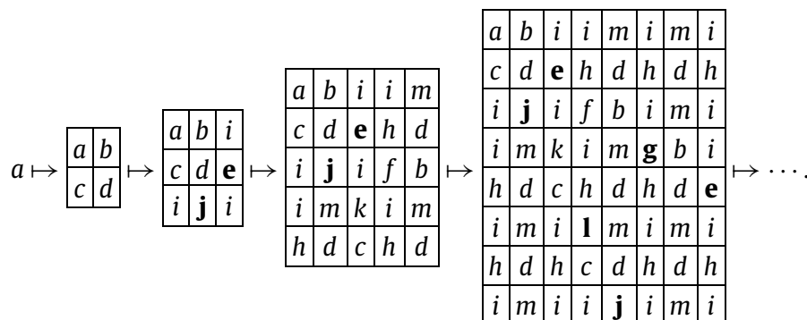
Fig. 7 in Appendix A gives a colored version (with respect to the different symbols) of the first 50 \times 50 block associated with \varphi^\omega(a) .
