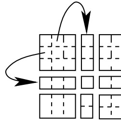
Fig. 3. Iteration of a shape-symmetric morphism.
