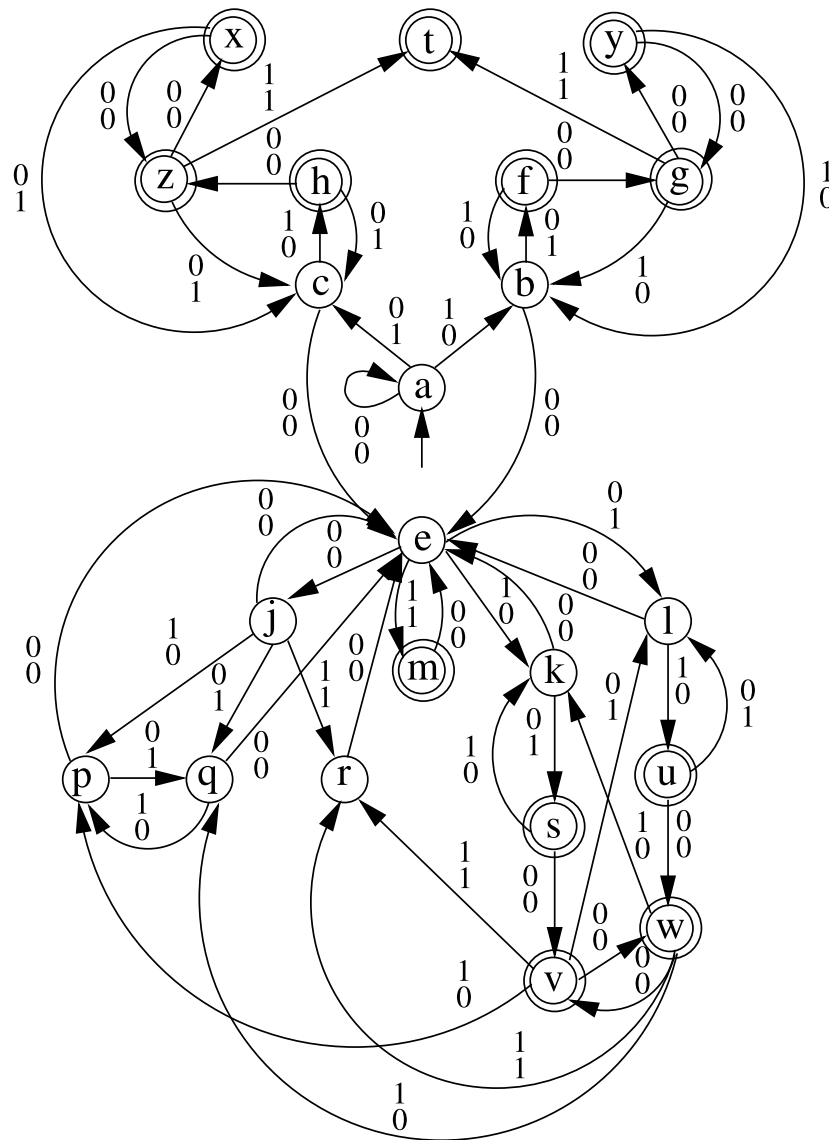
Fig. 5. The DFAO associated with \psi and \nu .
