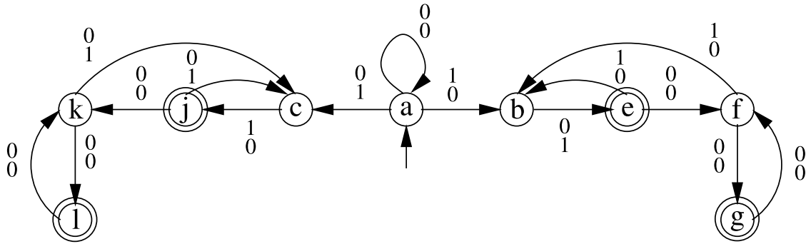
Fig. 4. Automaton accepting F -representations of (A_n, B_n) and (B_n, A_n) .
