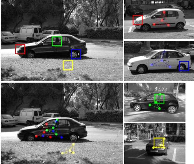
Figure 2. Voting process. Four patches from the test image (top left) are matched to database patches. The matching patches are shown with the corresponding color on the right column. Each match generates a vote in 6D pose space. We parameterize a point in pose space as a projection of designated points in 3D onto the image plane. These projections are shown here as dotted triangles. The red, green and blue votes correspond to a true detection, the cast pose votes are well clustered in pose space (bottom left) while the yellow match casts a false vote.
