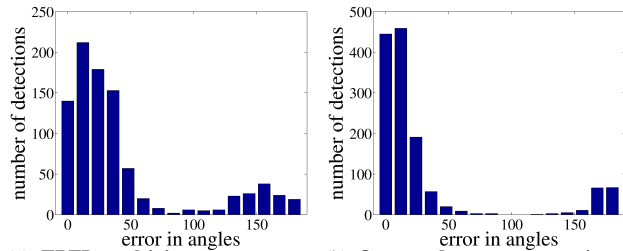
(a) EPFL multiview cars - pose estimation . A histogram of the angular errors in pose estimates. Our median angular error is 24.83 degrees. Computed on an 89.54% AP detection set. (b) Our car dataset - pose estimation . We achieve a median angular error of 10.4 degrees.
