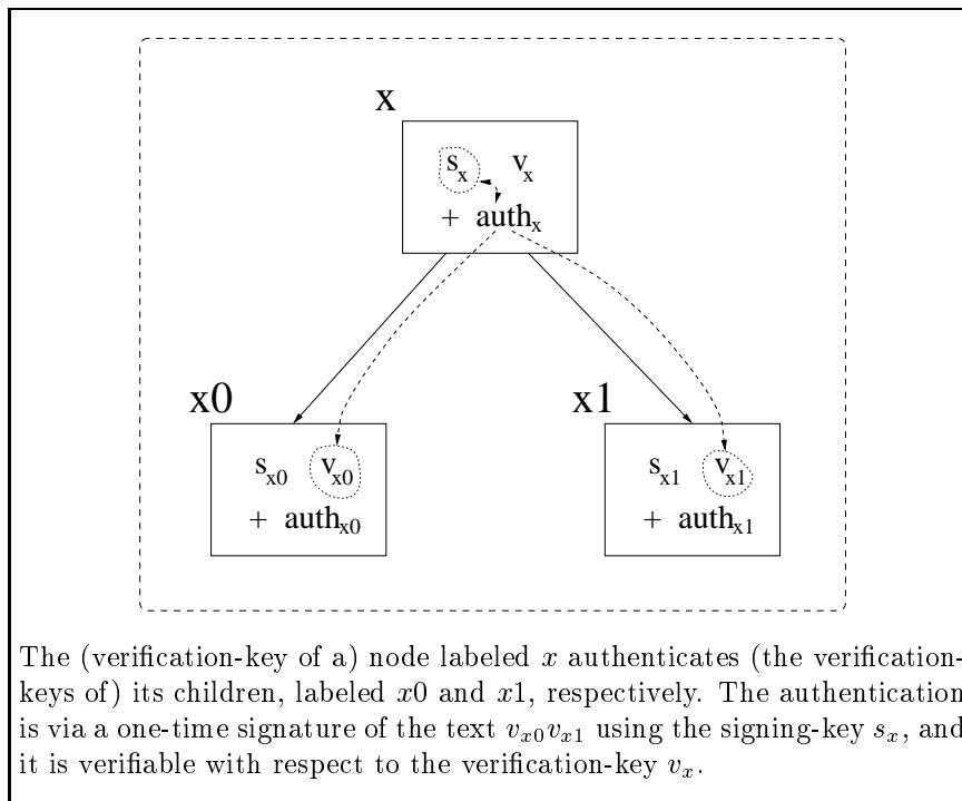
Figure 6.2: Authentication trees: the basic authentication step.
