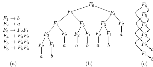
FIG. 1.1. (a) A context-free grammar generating the string abaababa . (b) The corresponding parse tree. (c) The acyclic graph defined by the grammar.
