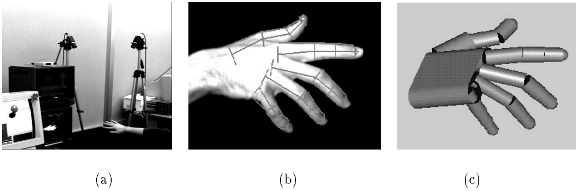
Figure 12: Hand tracking with the DigitEyes system (a) multi-camera setup (b) motion estimate superimposed on one of the two camera views (c) corresponding pose of 3-D hand model (from Rehg and Kanade [69], © 1994 Springer-Verlag).
