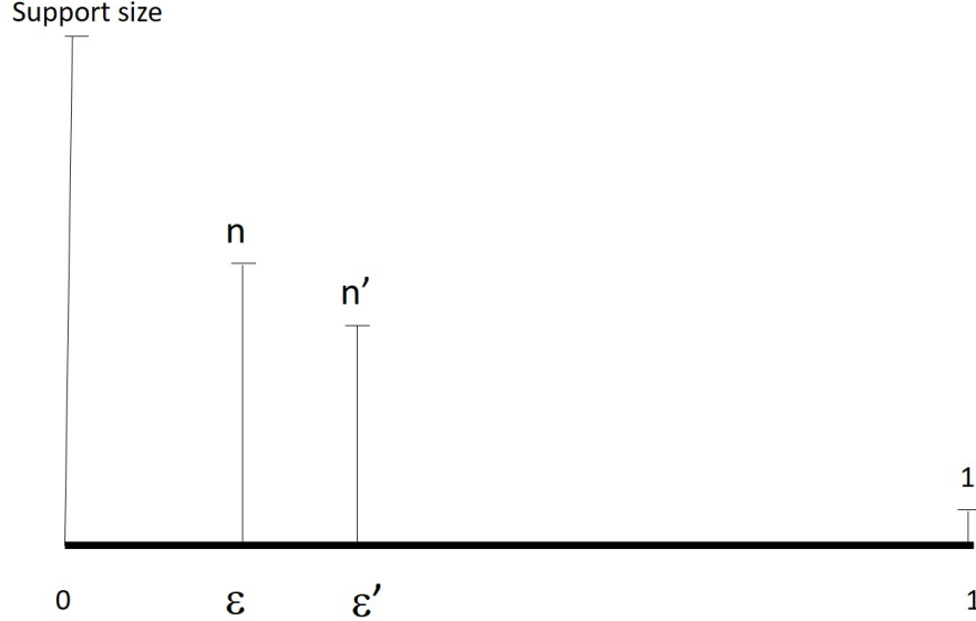
Figure 1: Showing n = \text{ess}_\epsilon(\mathcal{D}) and n' = \text{ess}_{\epsilon'}(\mathcal{D}) , for \epsilon < \epsilon' .
