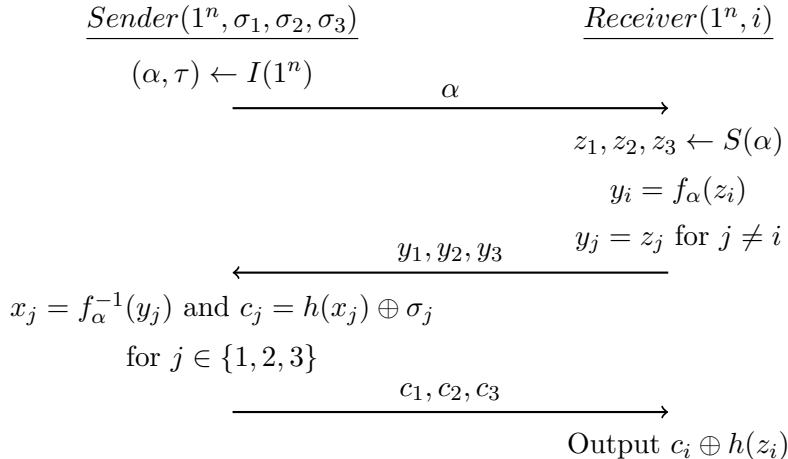
Figure 3: The EGL protocol for 1-out-of-3 Oblivious Transfer
