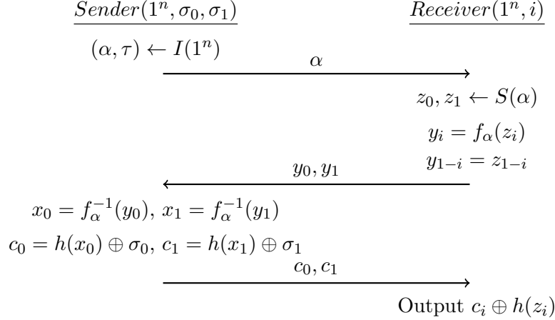
Figure 2: The EGL protocol for 1-out-of-2 Oblivious Transfer
